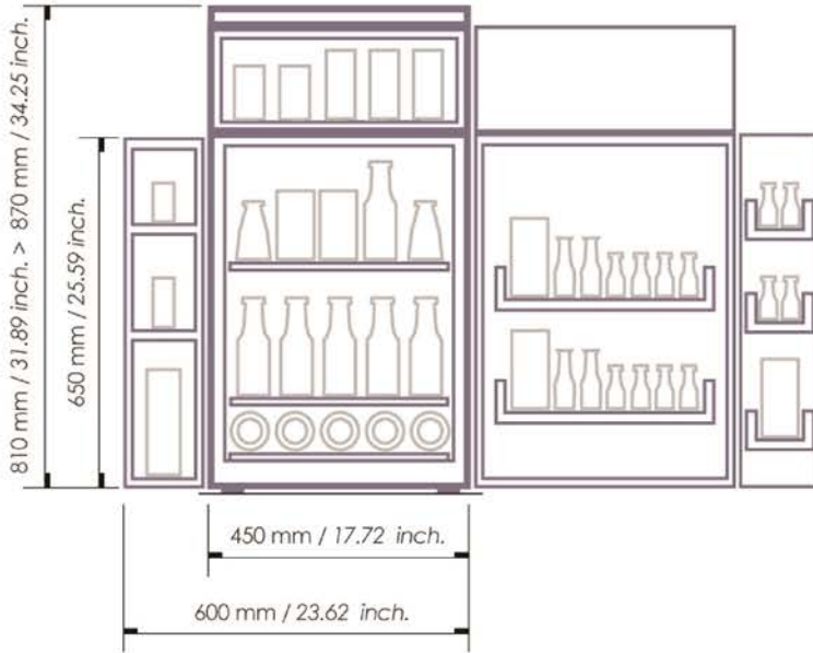
Integrated dry sections available with wooden door versions
